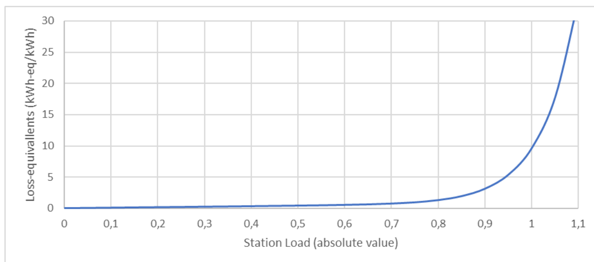
Figure 1. The curve in the diagram represents ideal energy losses (category 2.1) at low station loads and forward-looking costs (category 4.1) expressed as loss equivalents at high station loads.
